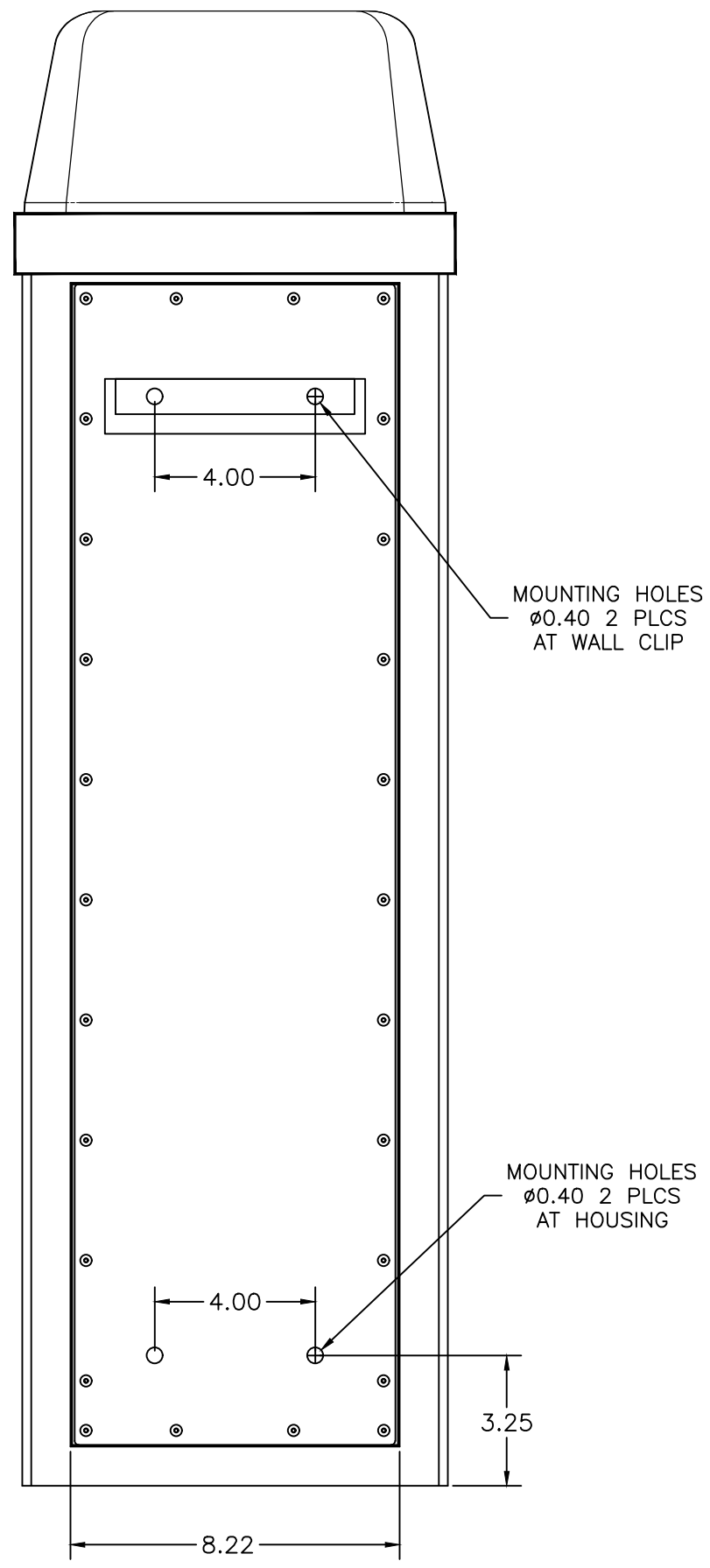
BACK VIEW SCALE 1:2
