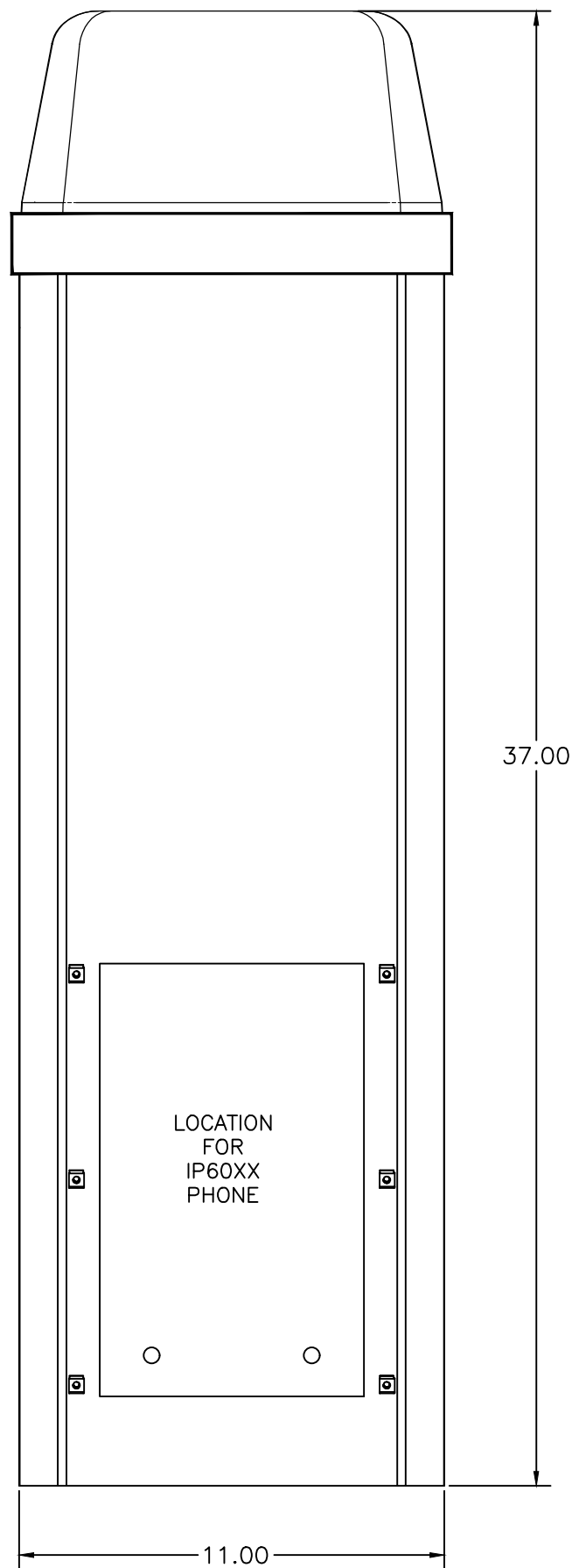
FRONT VIEW SCALE 1:2
